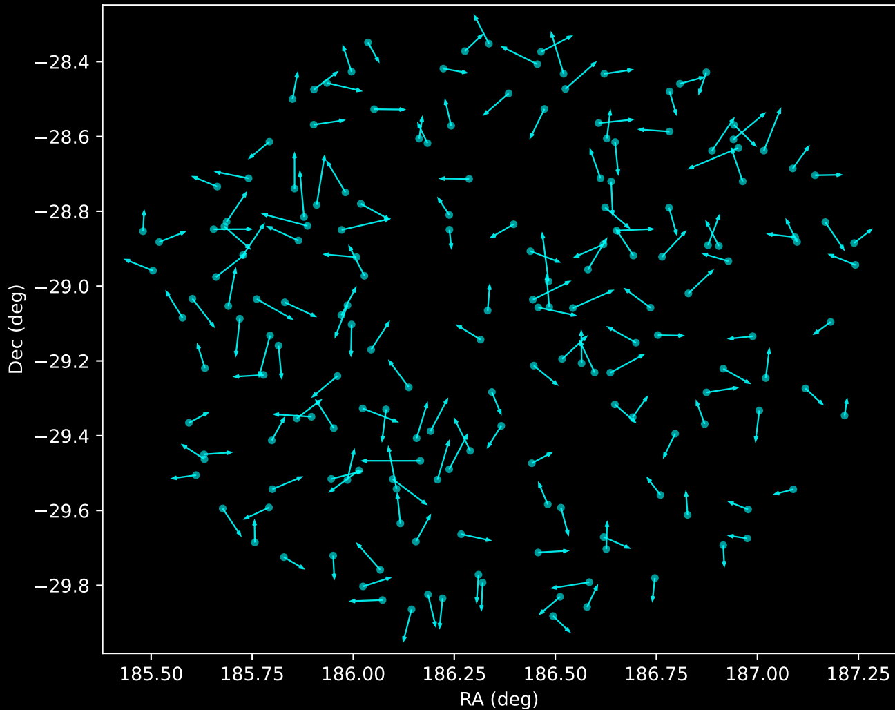
GALAH DR4 Noise Stream Proper Motion Vectors (n=179)
