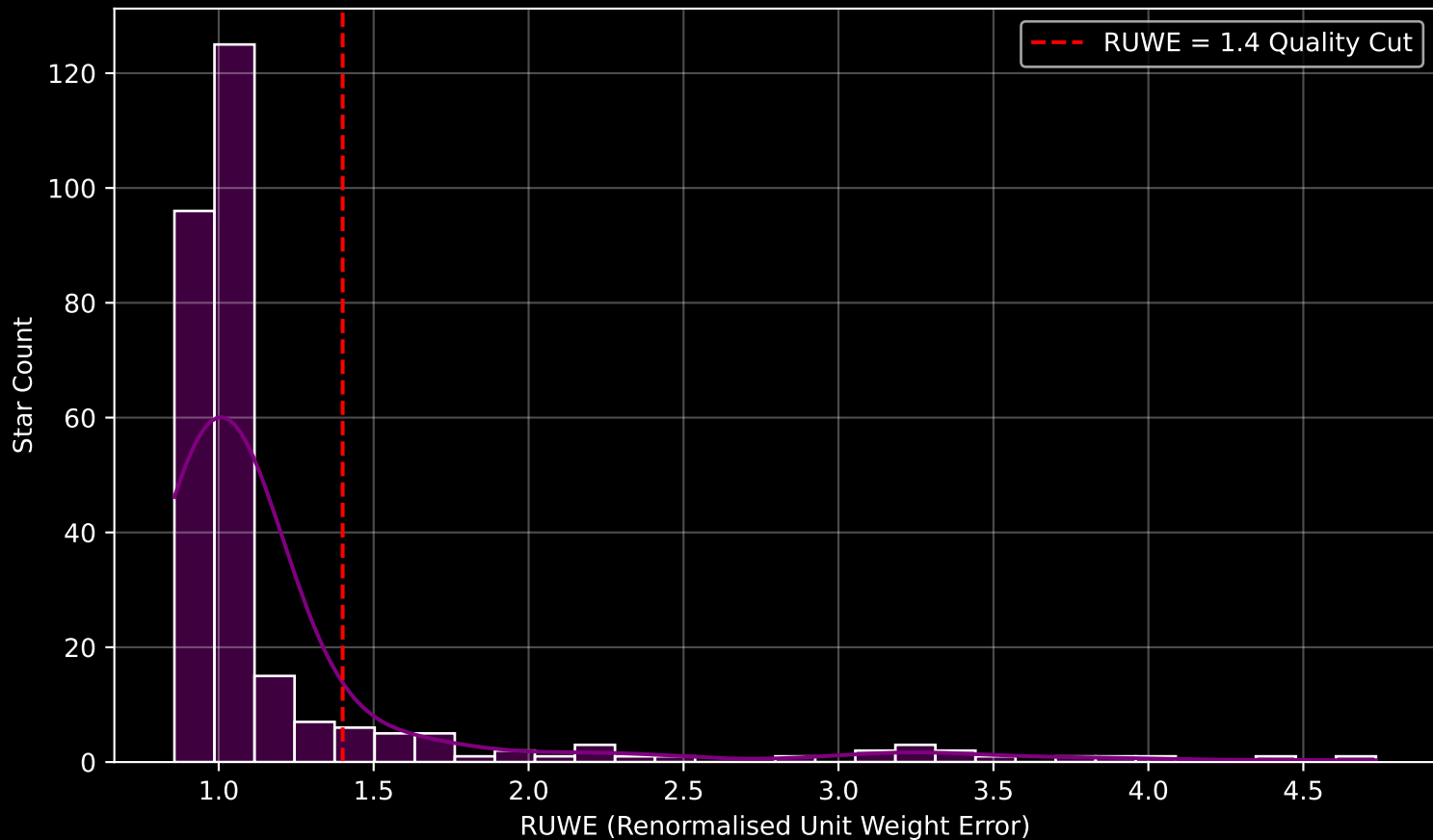
GALAH DR4 Field [1316] RUWE Distribution (n= 282)
