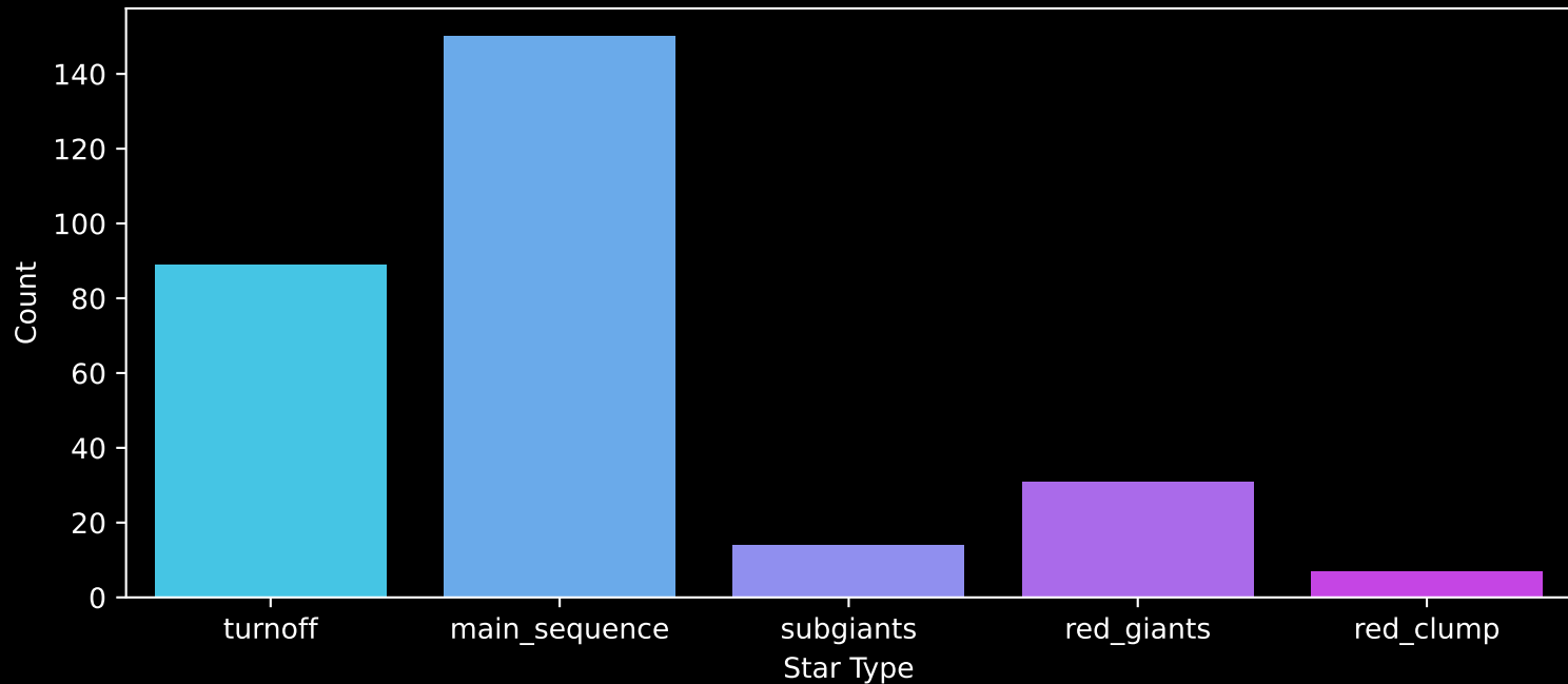
GALAH DR4 Field: [1316] Count plot of Star Type
